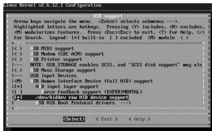
Figure 4-58. USB support menu
