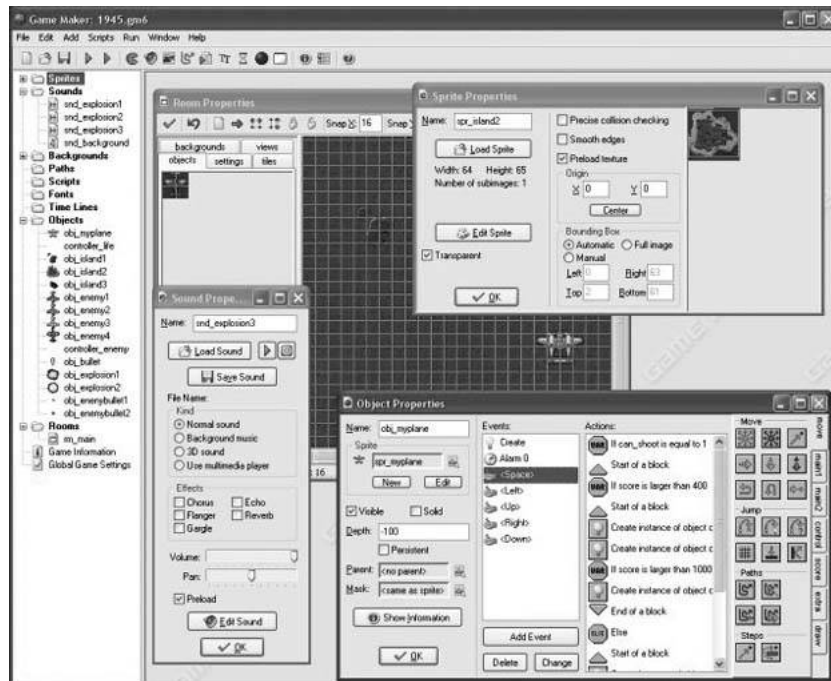
Figure 8-10. Game Maker's interface
