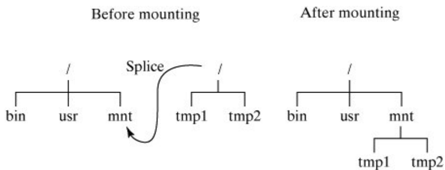
Figure 13-21. Mounting directories.
