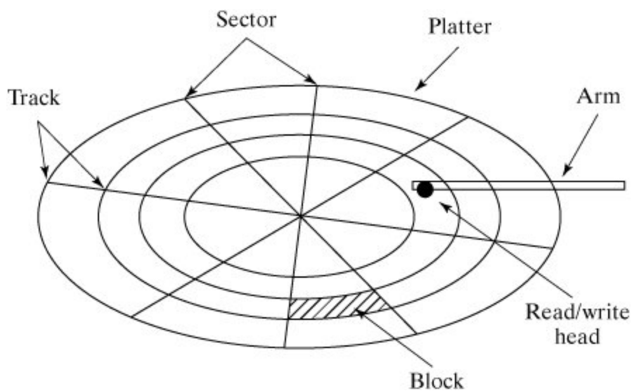
Figure 13-9. Disk architecture.
