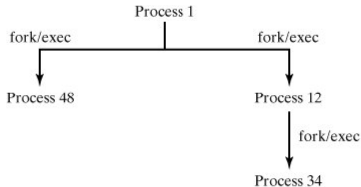
Figure 13-22. Process hierarchy.
