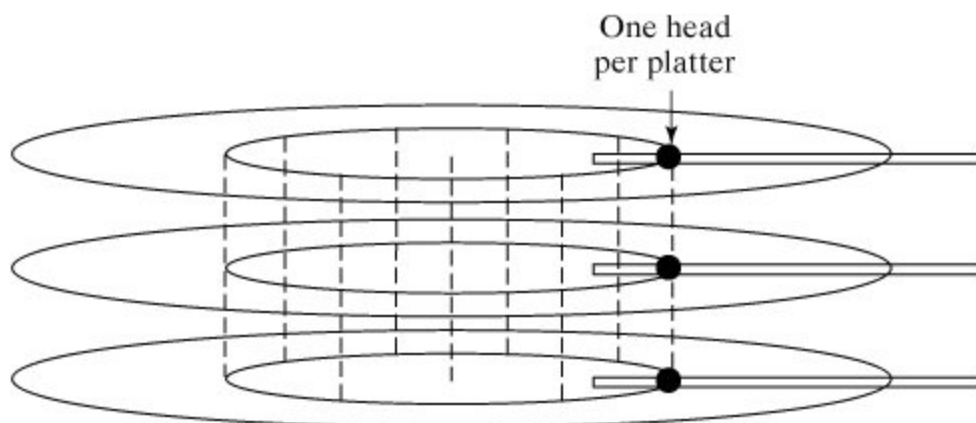
Figure 13-10. A multiplatter architecture.
