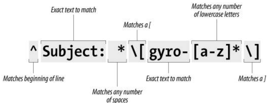
Figure 19-26. Regular expression with more parts
