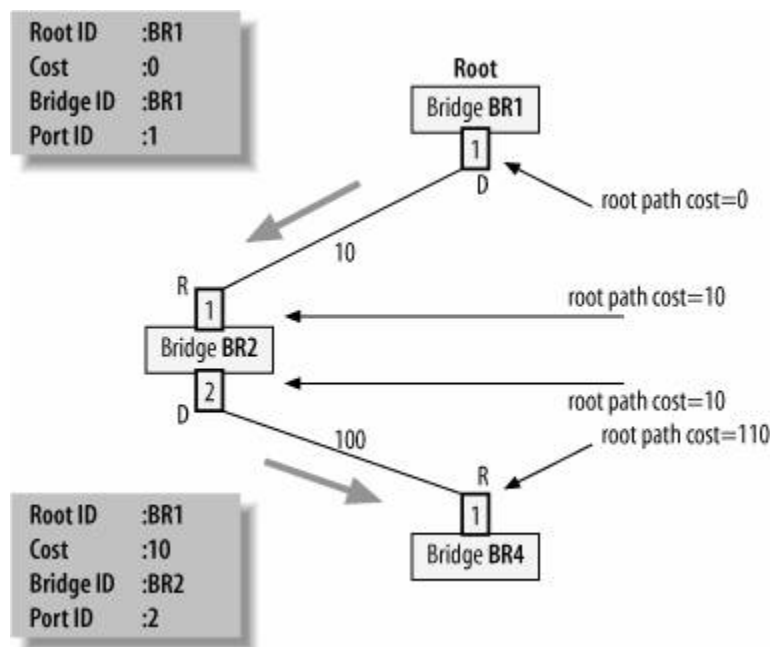
Figure 15-12. Updating the root path cost
