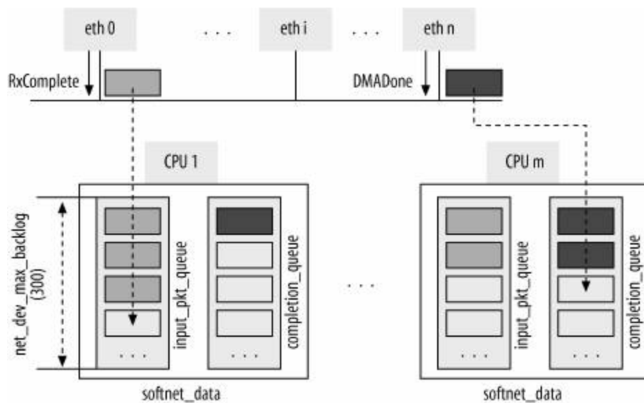
Figure 10-4. CPU's ingress queues
