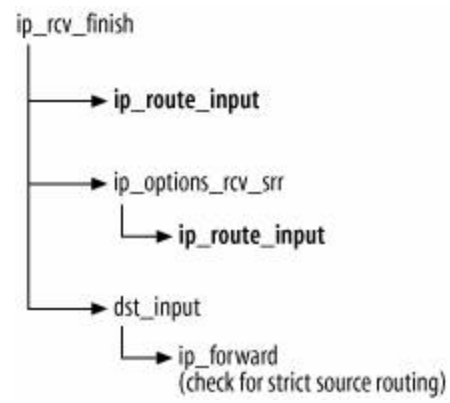
Figure 35-13. Source routing for ingress traffic
