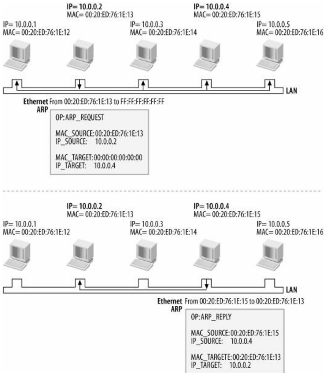
Figure 28-2. Example of ARP usage
