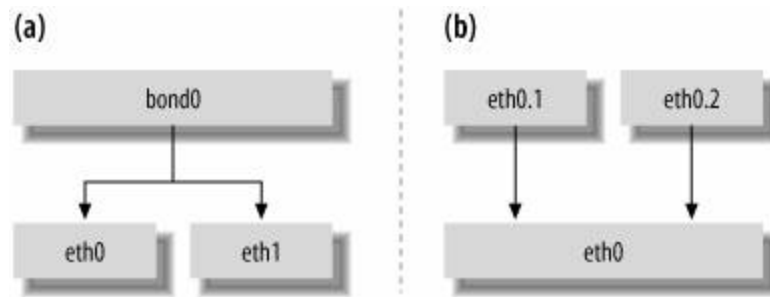
Figure 8-9. a) Bonding interface b) VLAN interfaces
