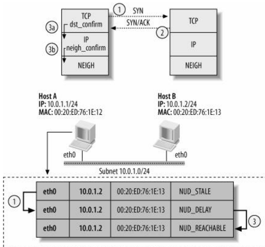
Figure 26-14. Example of external neighbor reachability confirmation
