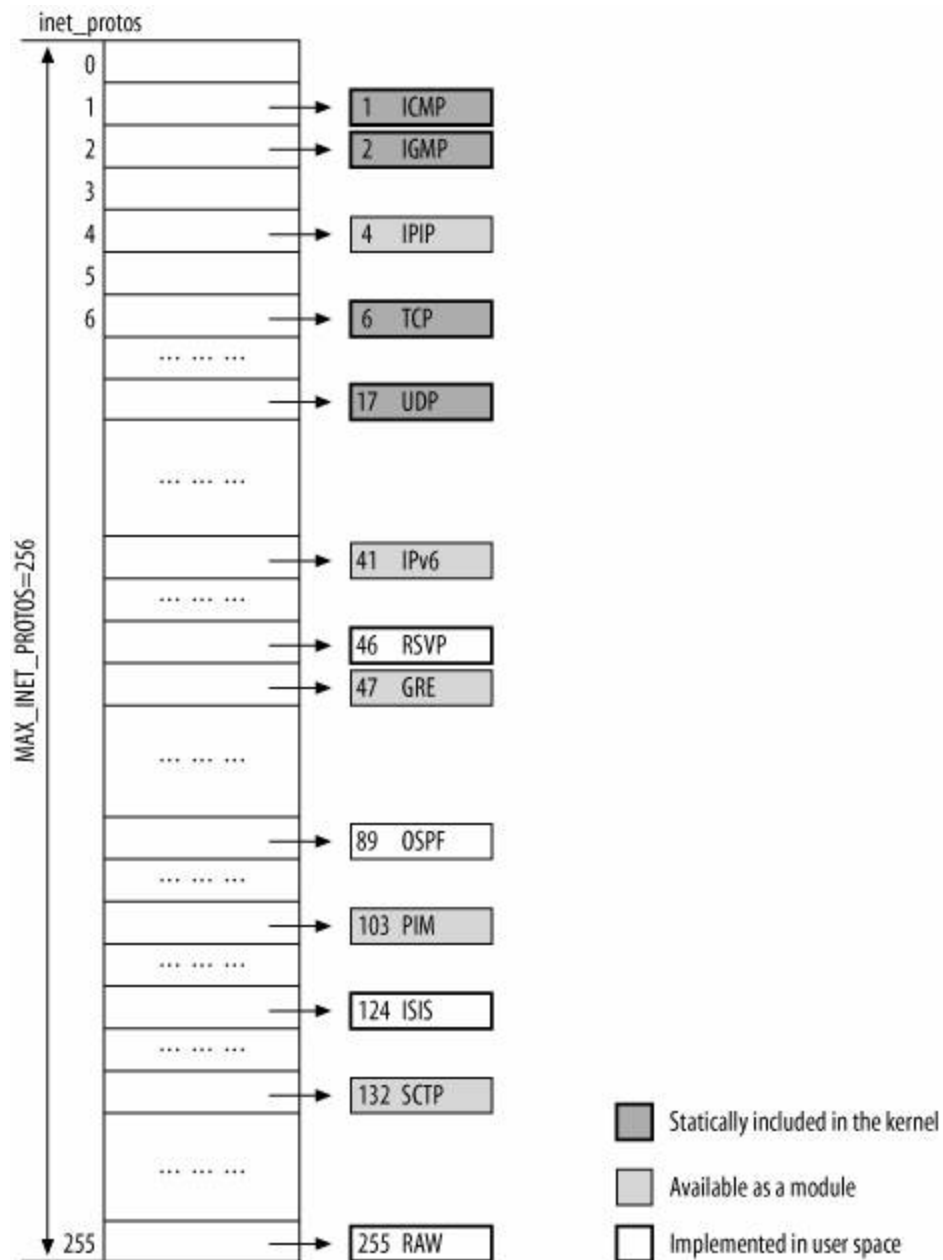
Figure 24-2. IPv4 protocol table
