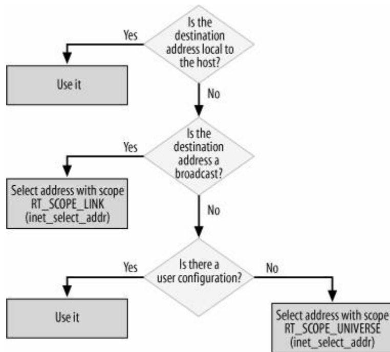
Figure 35-6. Selection of rt_spec_dst
