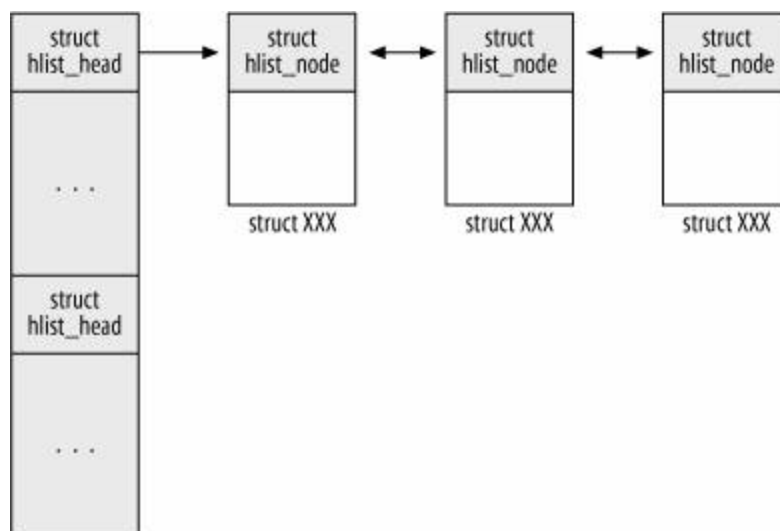
Figure 32-2. Generic hash table and use of lists
