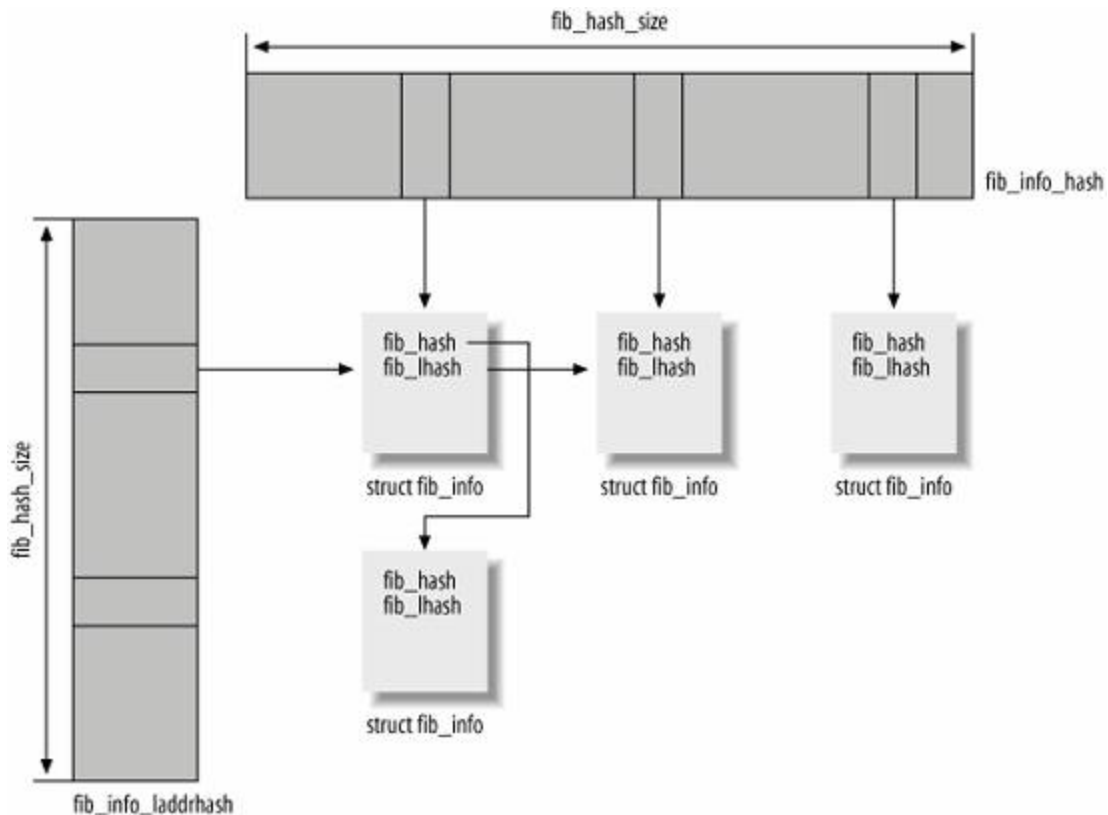
Figure 34-2. fib_info structures' organization
