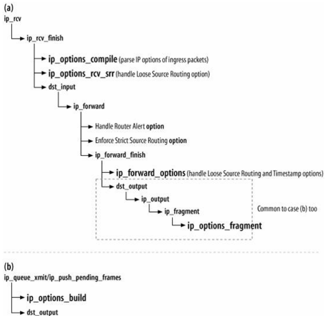
Figure 19-3. (a) Ingress packets; (b) locally generated packets
