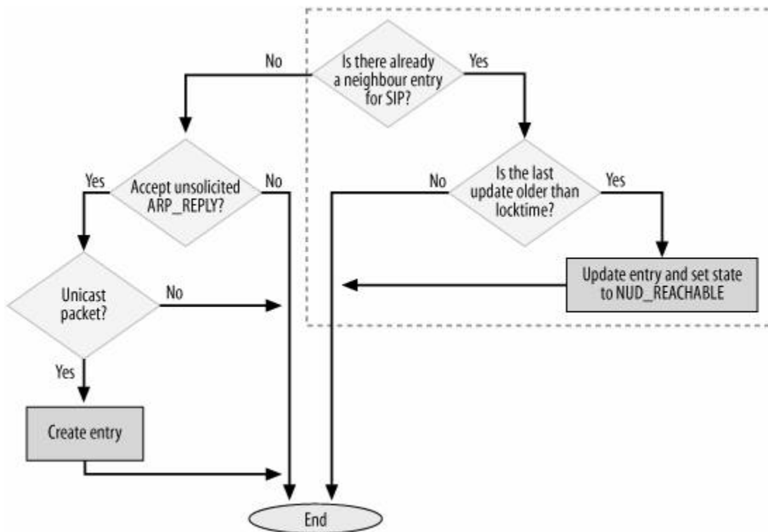
Figure 28-18. ARPOP_REPLY handling by arp_process
