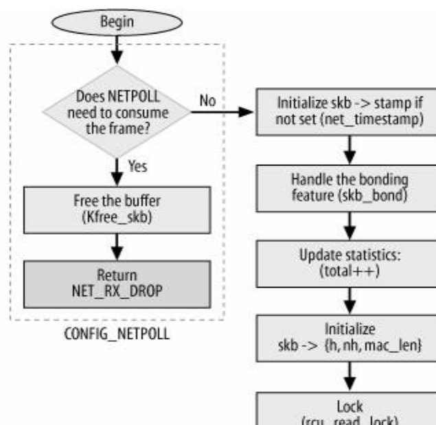
Figure 10-7. The netif_receive_skb function
