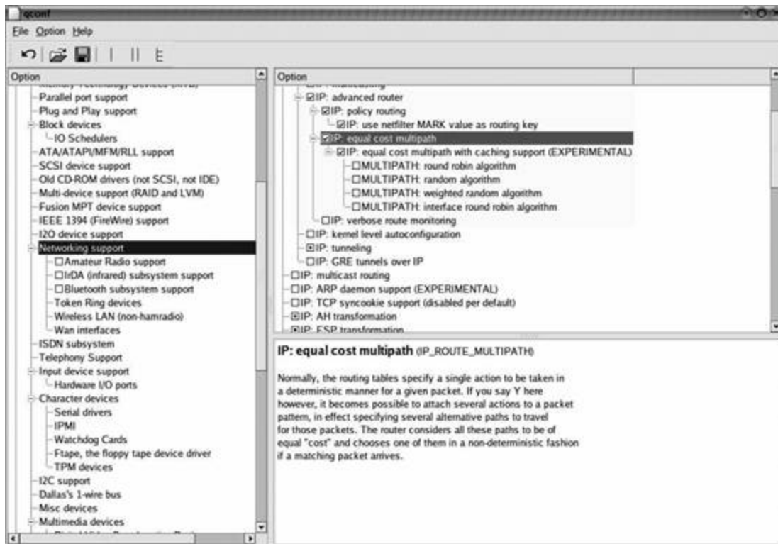
Figure 32-1. Kernel configuration (make xconfig)
