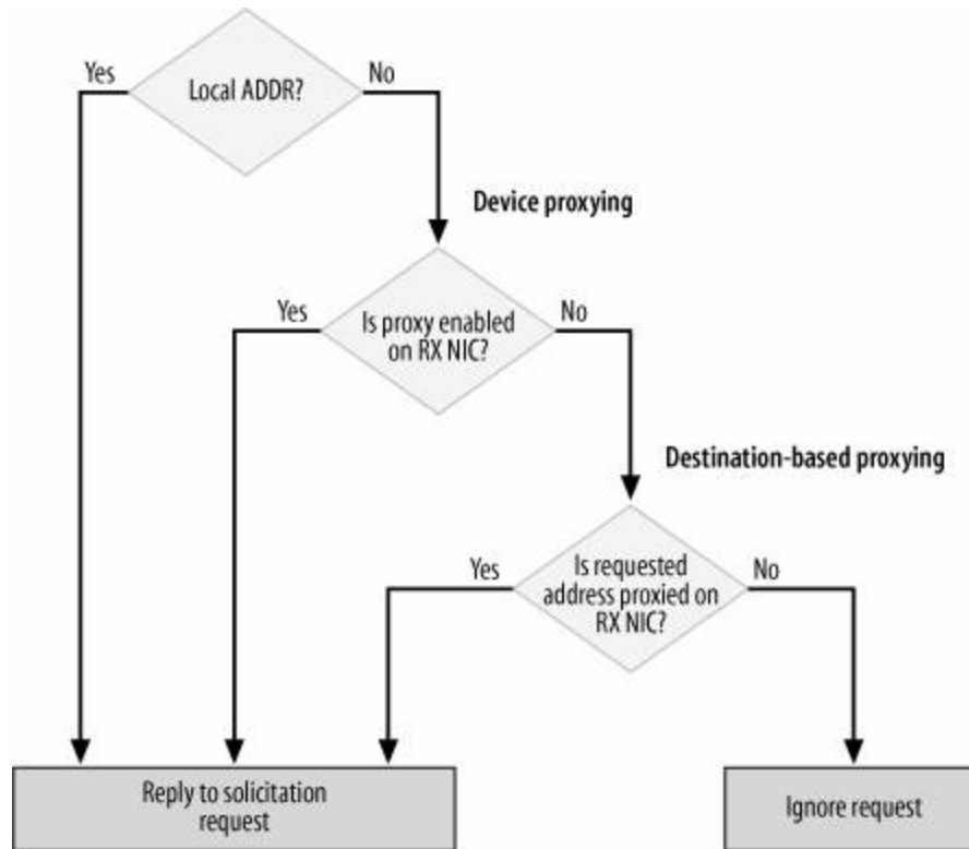
Figure 26-8. Priority between device and address proxying
