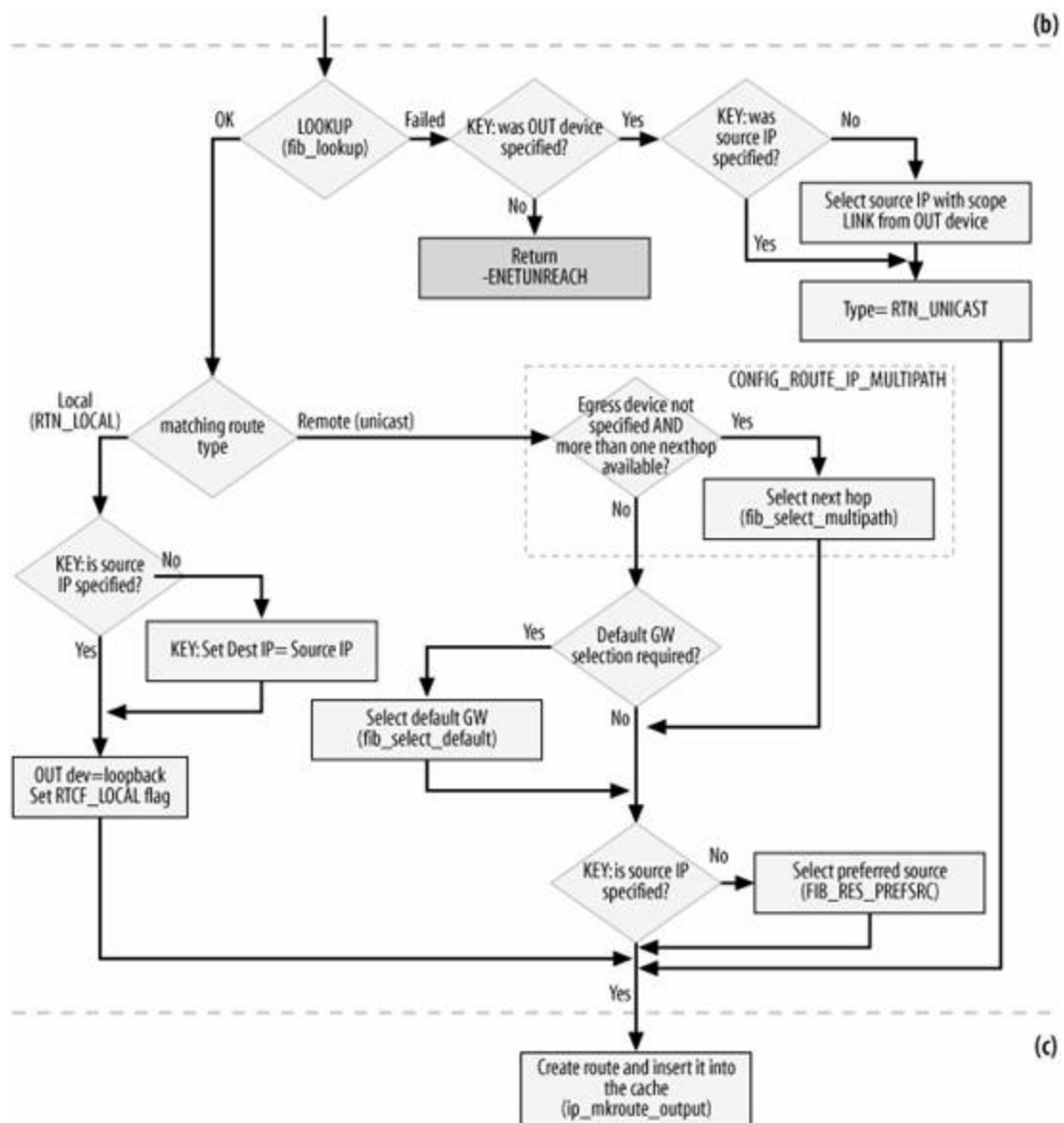
Figure 35-8b. p_route_output_slow function
