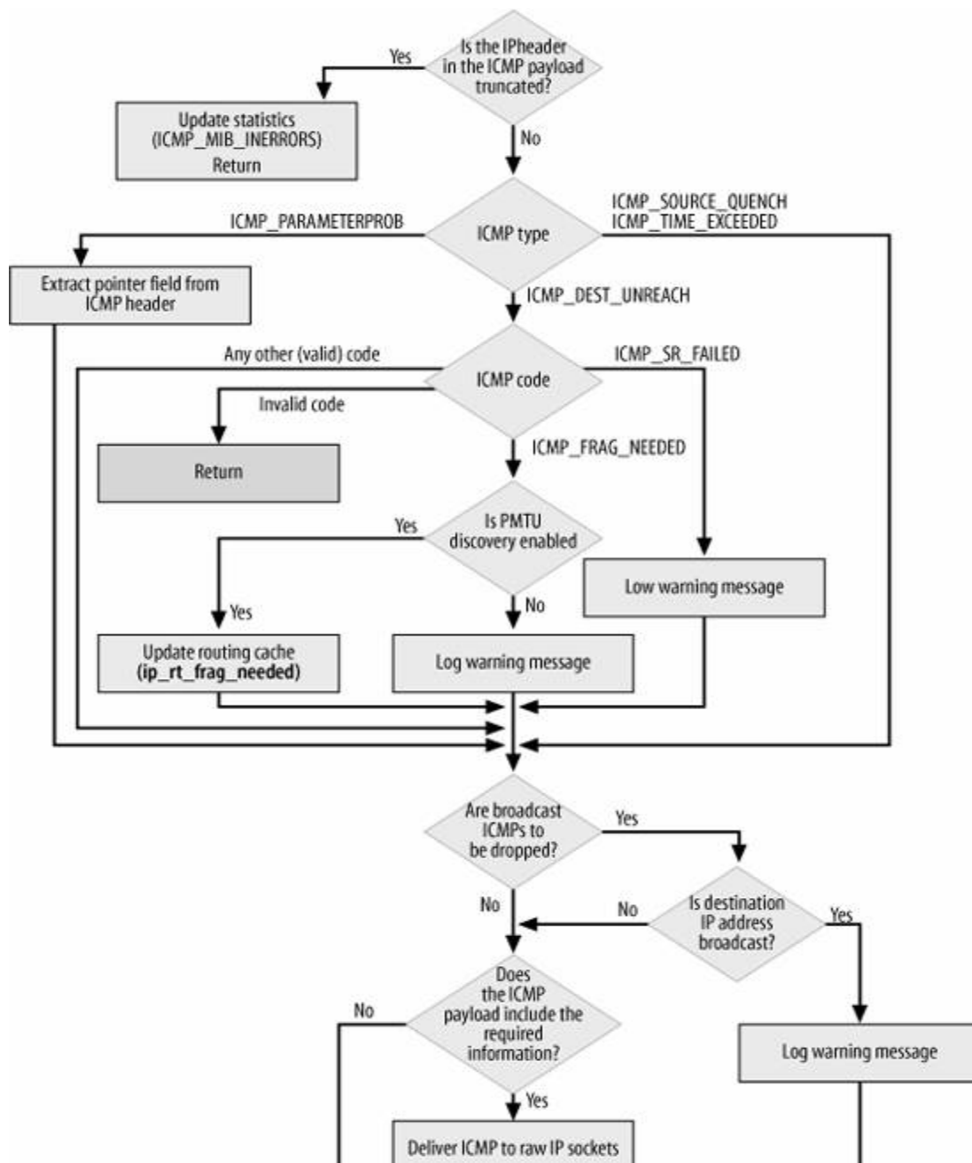
Figure 25-13. icmp_unreach function
