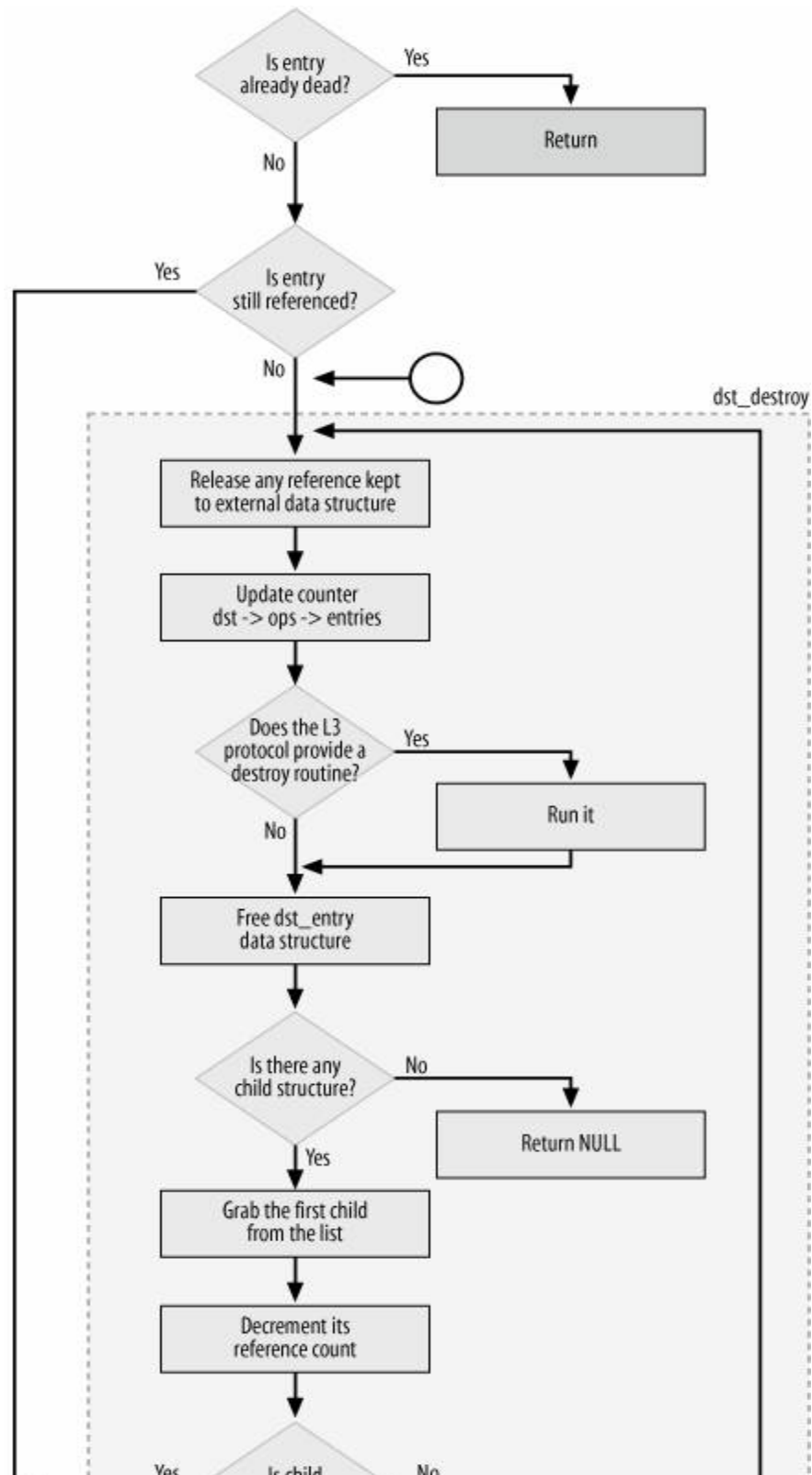
Figure 33-10a. dst_free function
