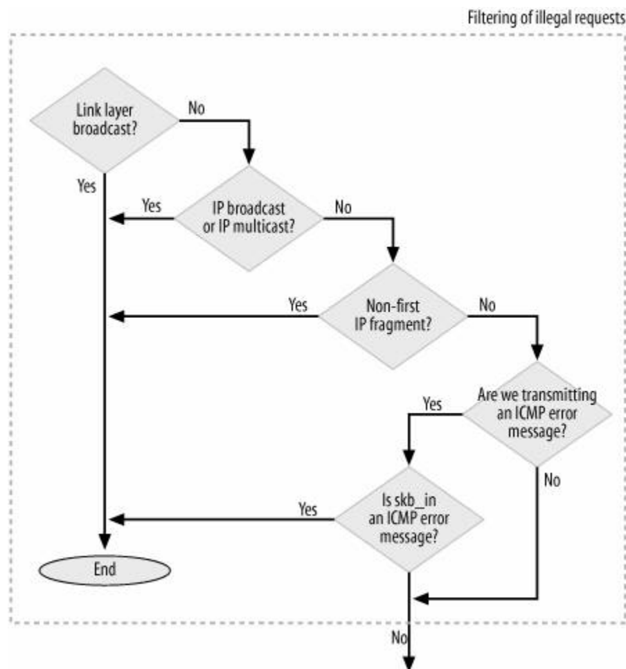
Figure 25-9a. icmp_send function
