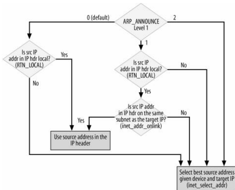
Figure 28-15. Selection of source IP in arp_solicit
