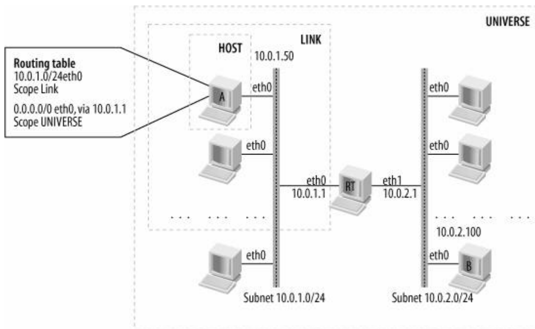
Figure 30-6. Simple network topology
