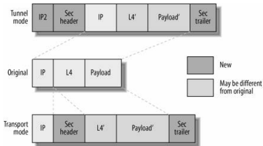
Figure 24-5. IPsec headers/trailers locations
