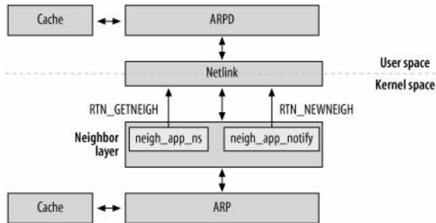
Figure 28-22. Interaction between ARP and arpd daemon
