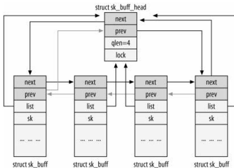
Figure 2-1. List of sk_buff elements
