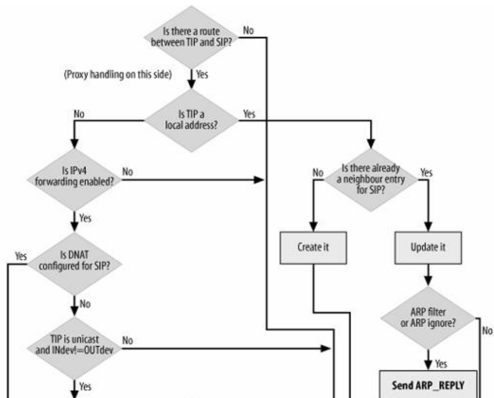
Figure 28-17. ARPOP_REQUEST handling by arp_process
