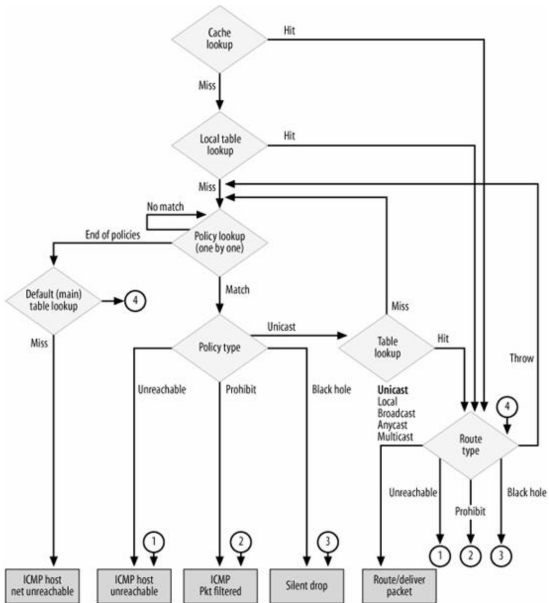
Figure 31-2. Policy routing lookup
