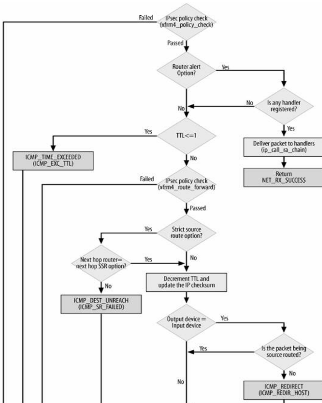
Figure 20-1. ip_forward function
