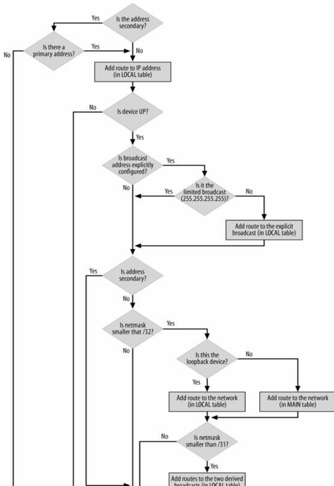
Figure 32-7. fib_add_ifaddr function
