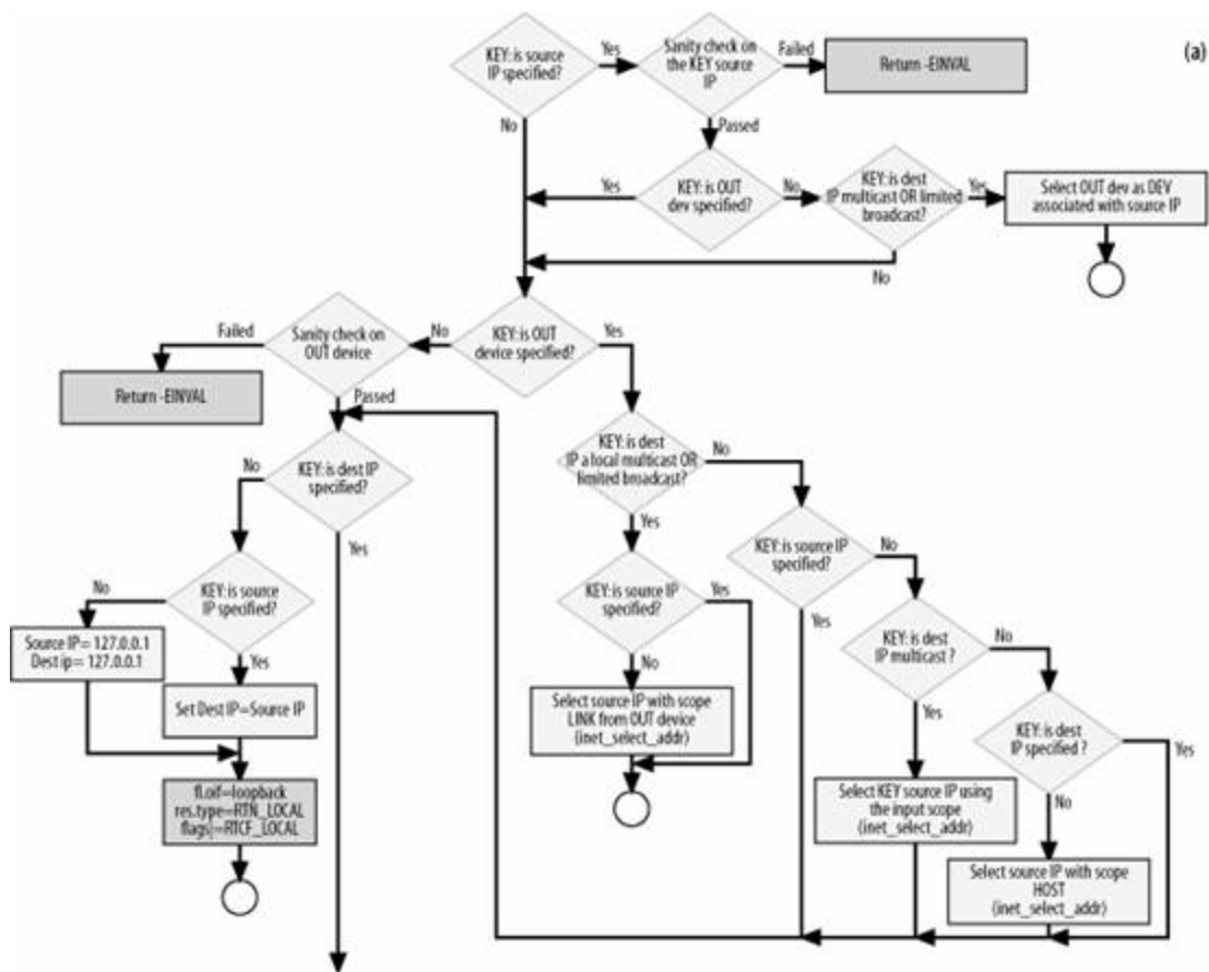
Figure 35-8a. ip_route_output_slow function
