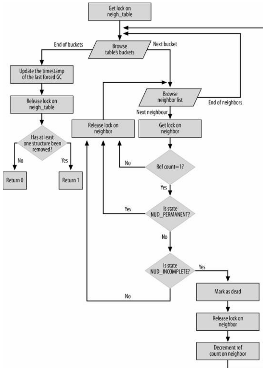
Figure 27-7. neigh_forced_gc function
