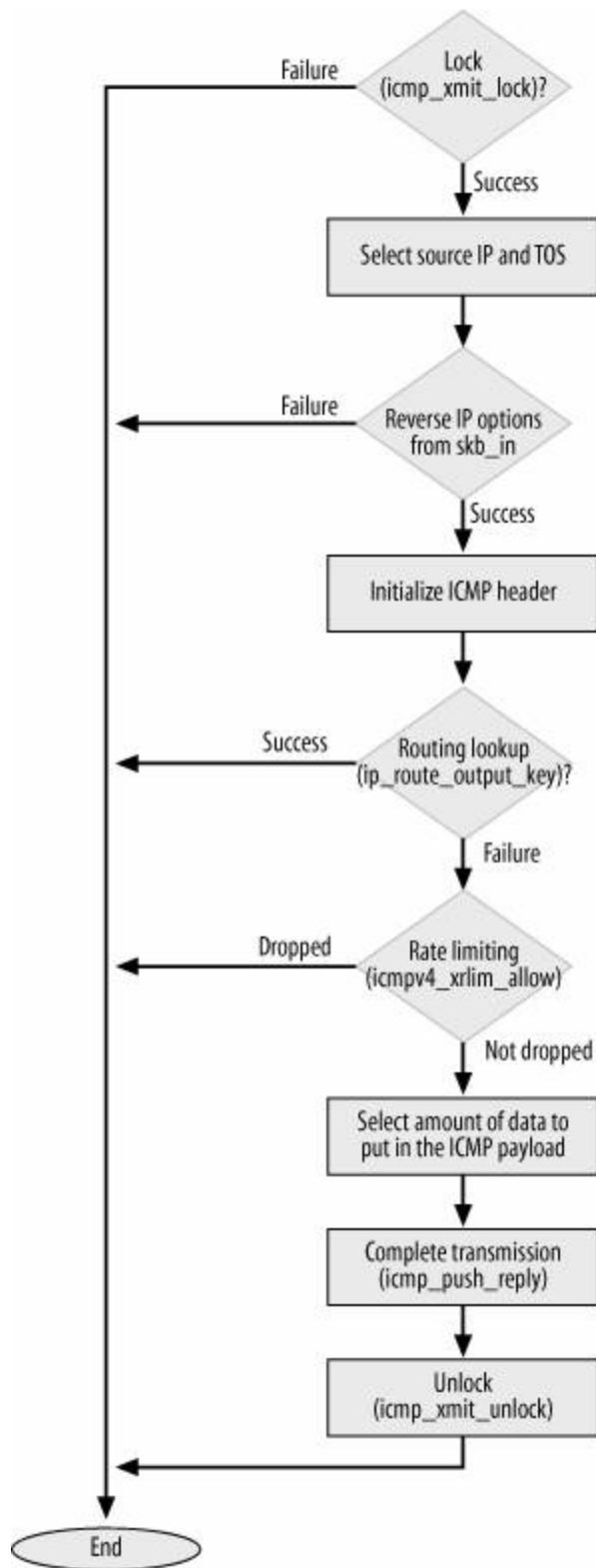
Figure 25-9b. icmp_send function
