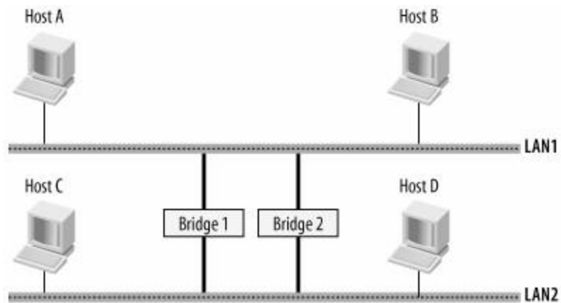
Figure 14-7. Redundant bridges
