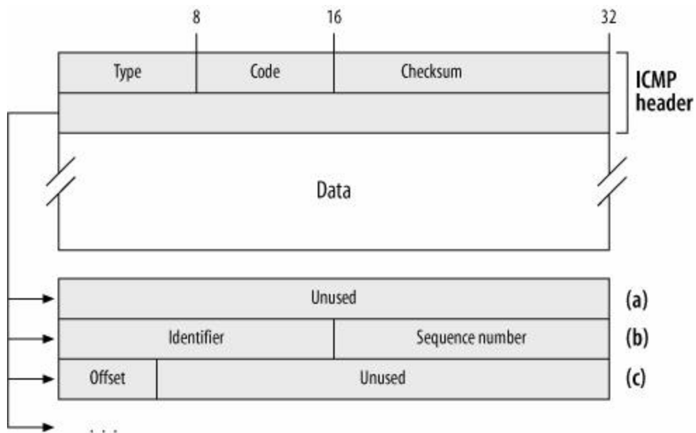
Figure 25-1. ICMP header
