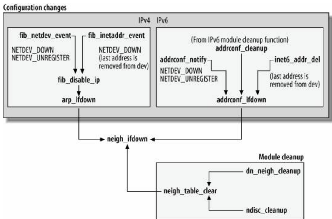
Figure 27-11. Contexts where neigh_ifdown is called
