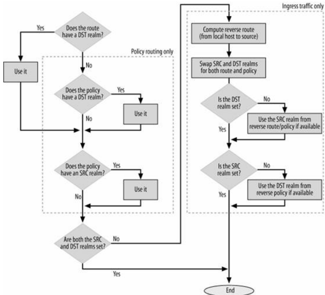
Figure 31-8. Logic used to compute the routing tag
