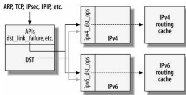
Figure 33-6. dst_ops interface
