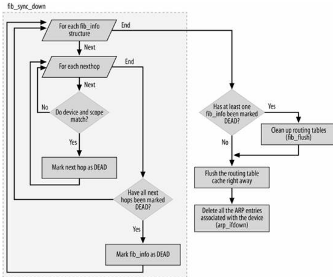
Figure 32-6. fib_disable_ip function
