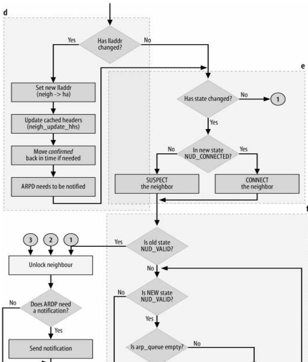
Figure 27-5b. neigh_update function
