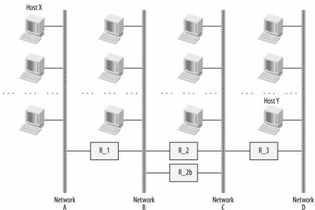
Figure 18-6. Example of IP source routing
