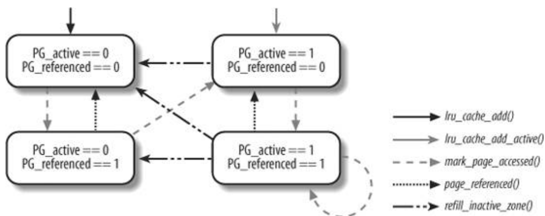
Figure 17-4. Moving pages across the LRU lists
