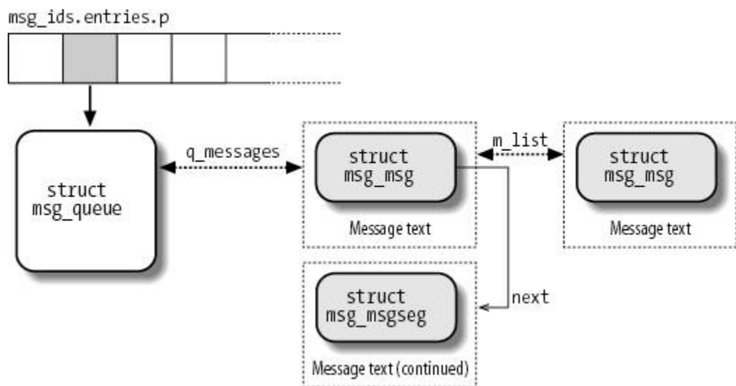
Figure 19-2. IPC message queue data structures
