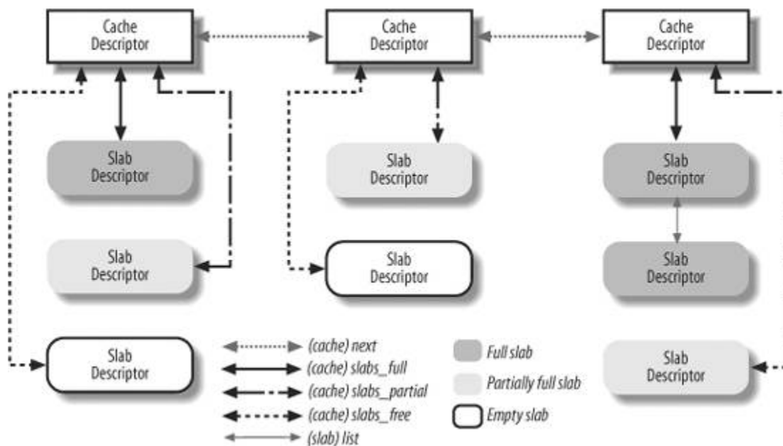
Figure 8-4. Relationship between cache and slab descriptors
