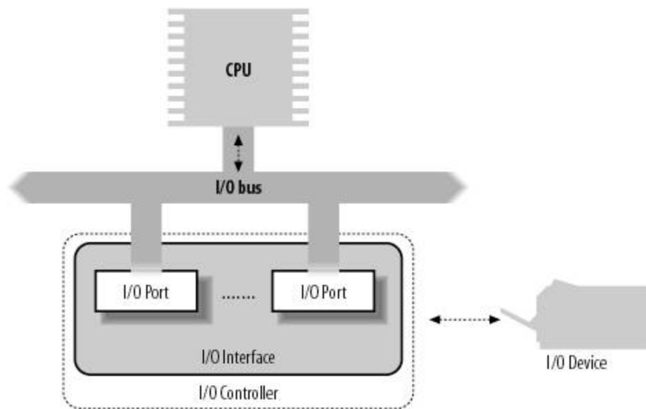
Figure 13-1. PC's I/O architecture
