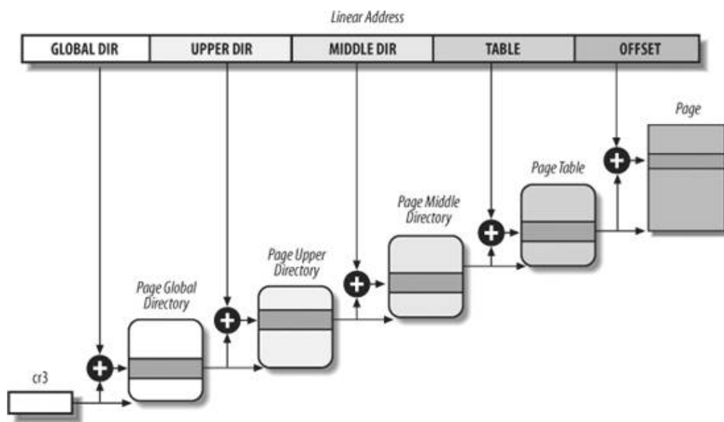
Figure 2-12. The Linux paging model
