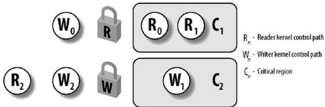
Figure 5-2. Read/write spin locks
