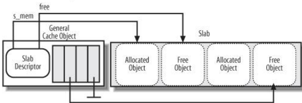
Slab with External Descriptors
