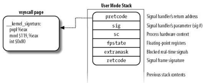
Figure 11-3. Frame on the User Mode stack
