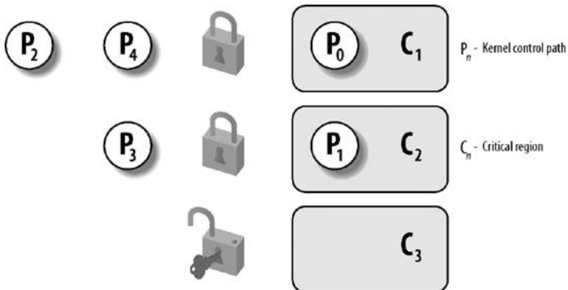
Figure 5-1. Protecting critical regions with several locks
