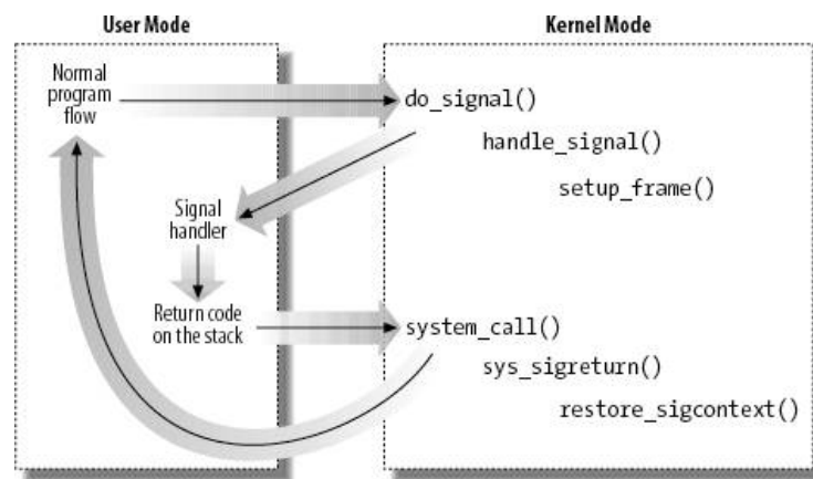
Figure 11-2. Catching a signal
