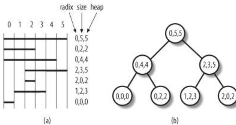
Figure 17-2. A simple example of priority search tree
