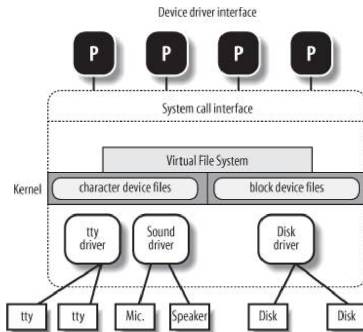
Figure 1-4. Device driver interface
