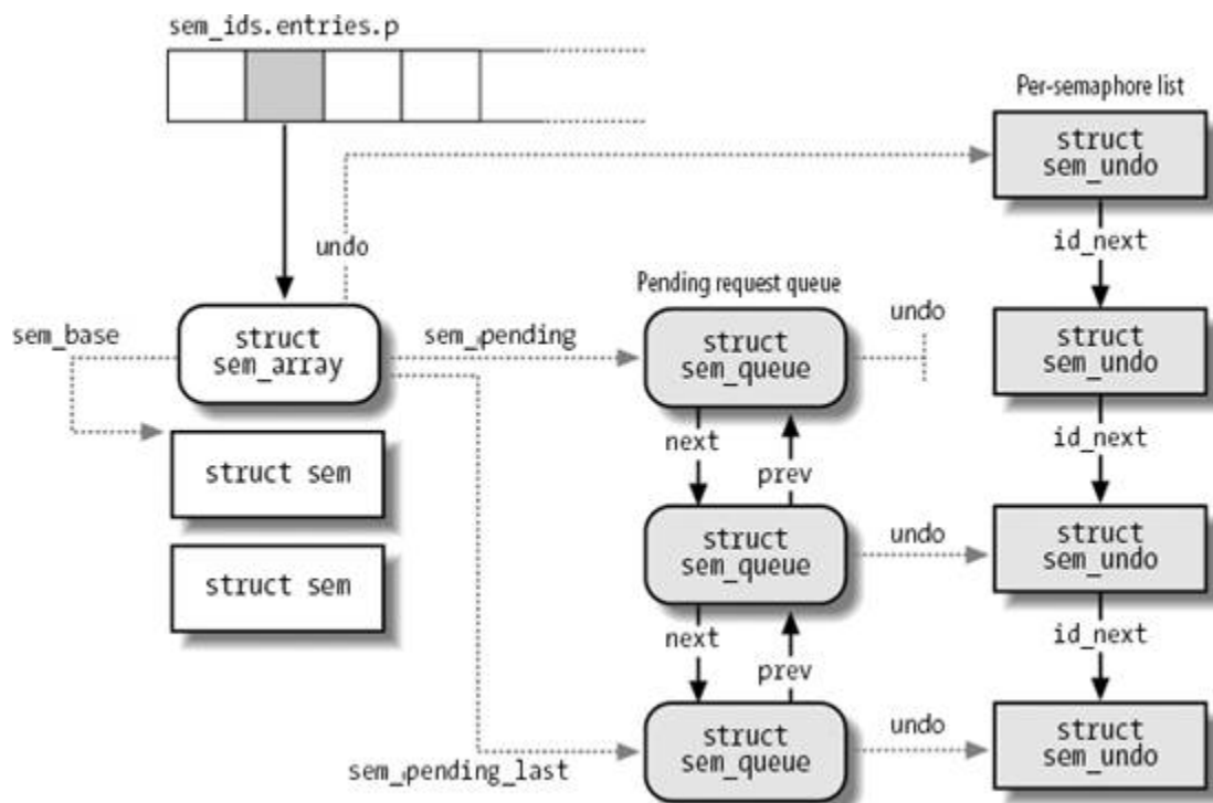
Figure 19-1. IPC semaphore data structures
