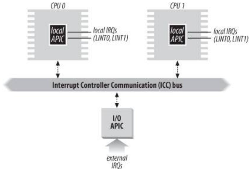
Figure 4-1. Multi-APIC system
