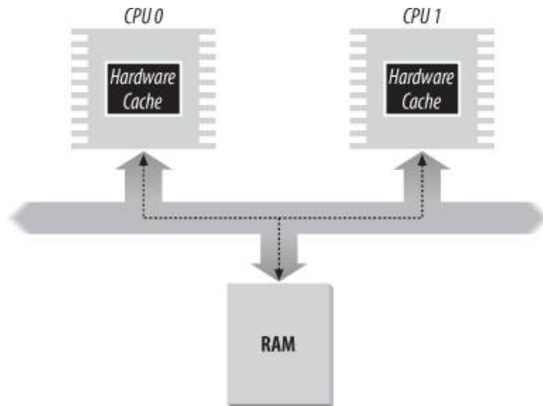
Figure 2-11. The caches in a dual processor
