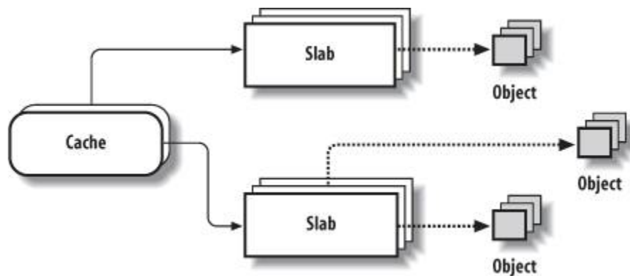
Figure 8-3. The slab allocator components
