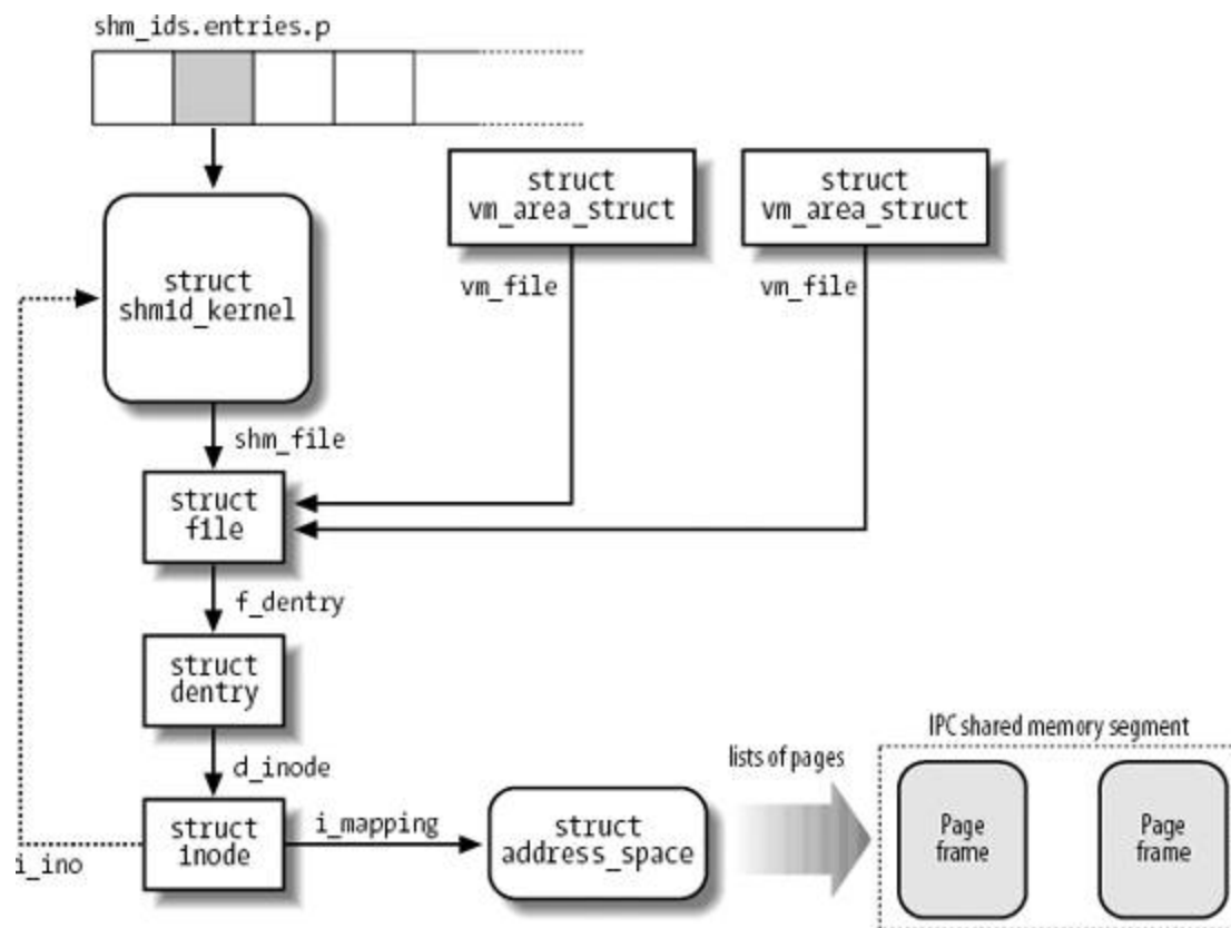
Figure 19-3. IPC shared memory data structures
