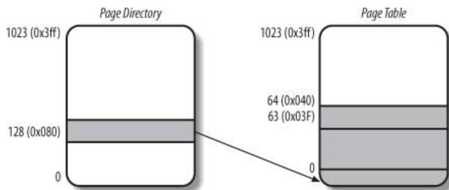
Figure 2-9. An example of paging
