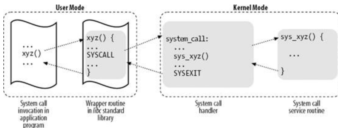
Figure 10-1. Invoking a system call
