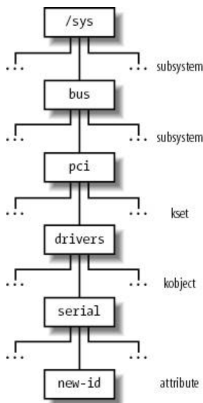
Figure 13-3. An example of device driver model hierarchy
