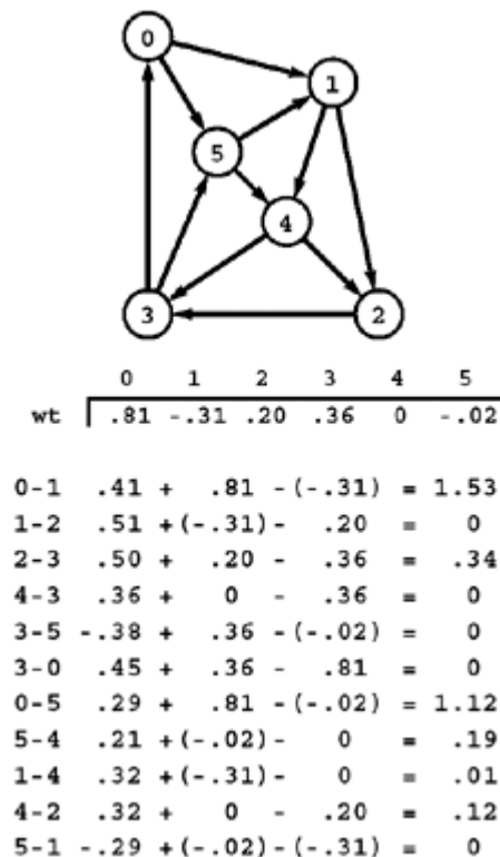
Figure 21.32. All shortest paths in a reweighted network
