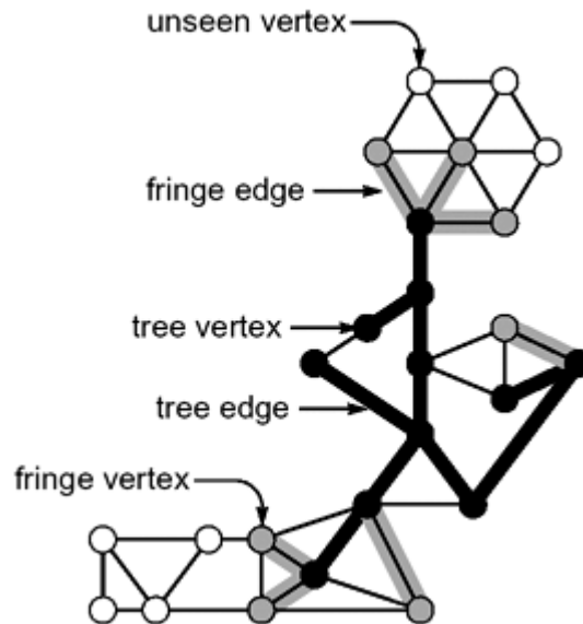
Figure 18.27. Graph search strategies
