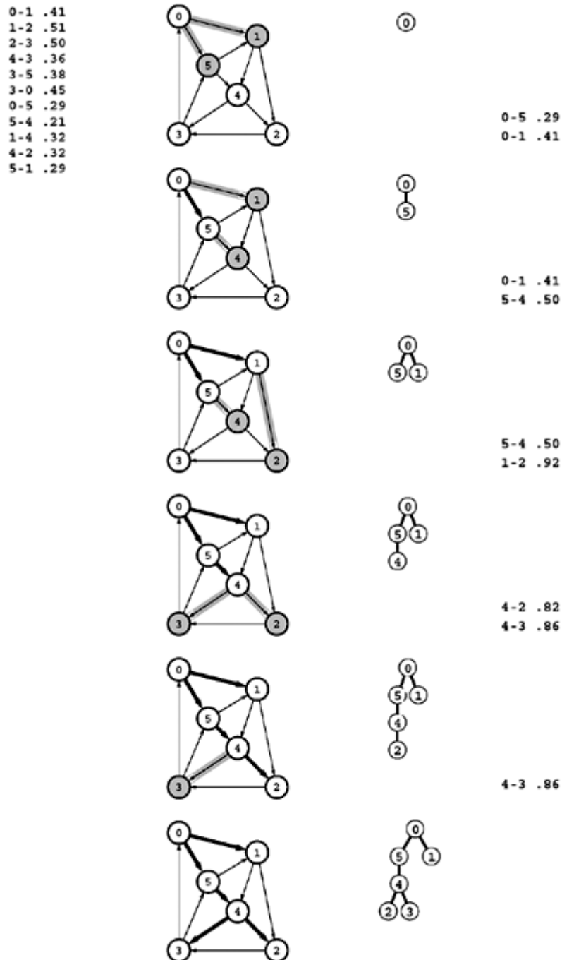
Figure 21.11. Shortest-paths spanning tree
