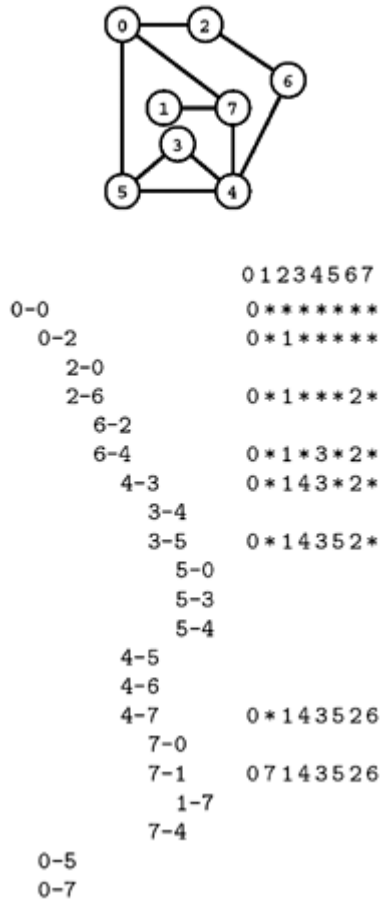
Figure 18.6. Depth-first search
