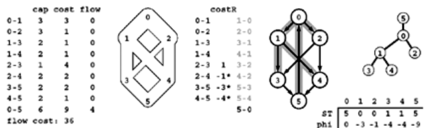
Figure 22.50. Residual networks and spanning trees (network simplex)
