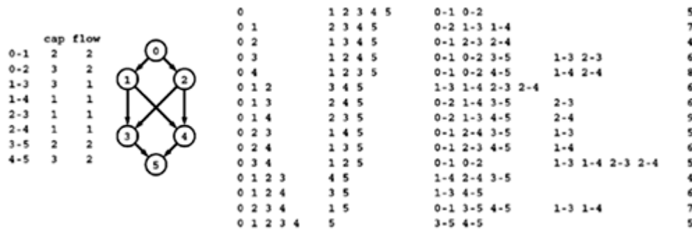
Figure 22.16. Residual networks (augmenting paths)
