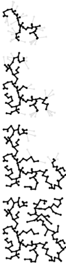
Figure 20.11. Fringe size for PFS implementation of Prim's algorithm
