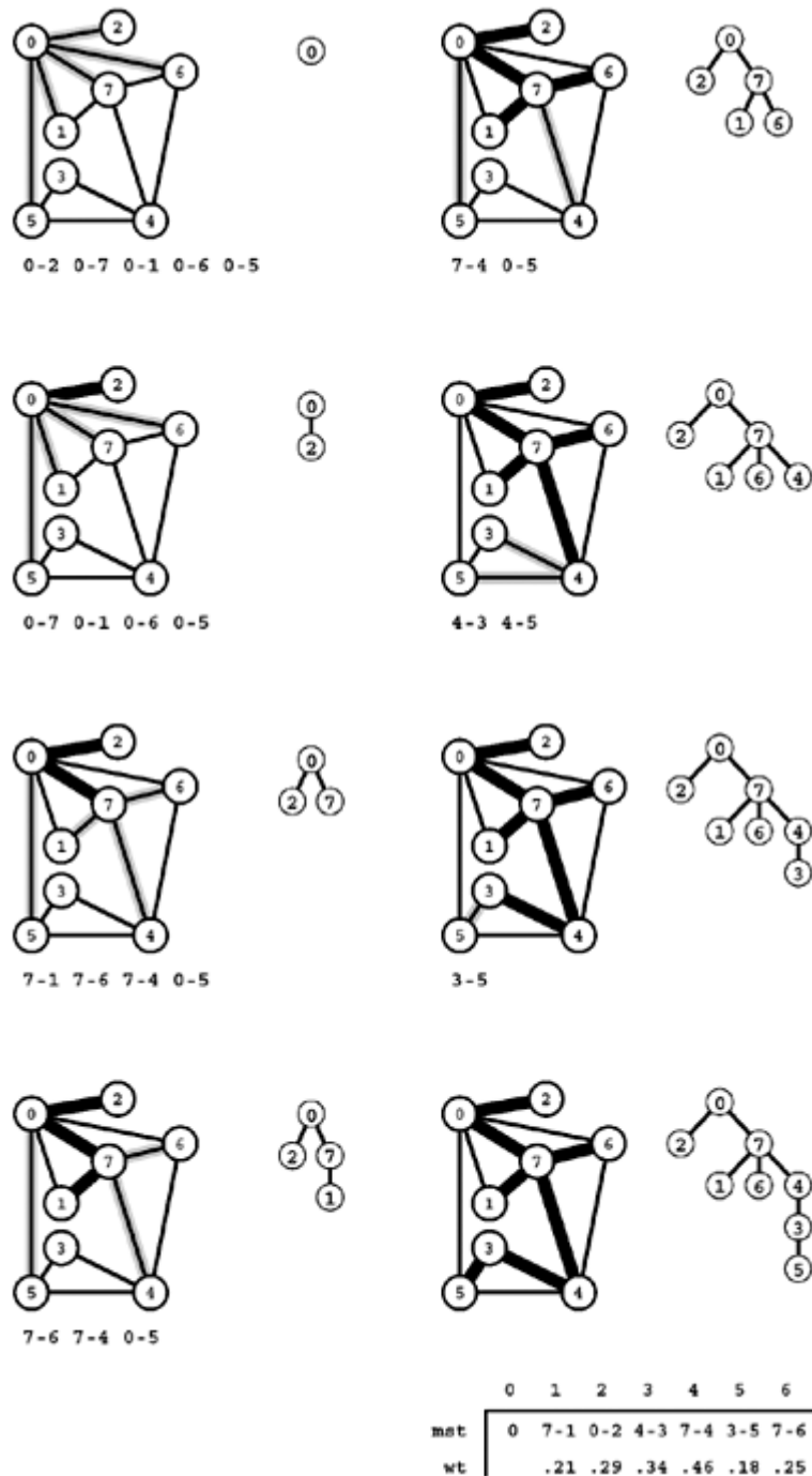
Figure 20.9. Prim's MST algorithm
