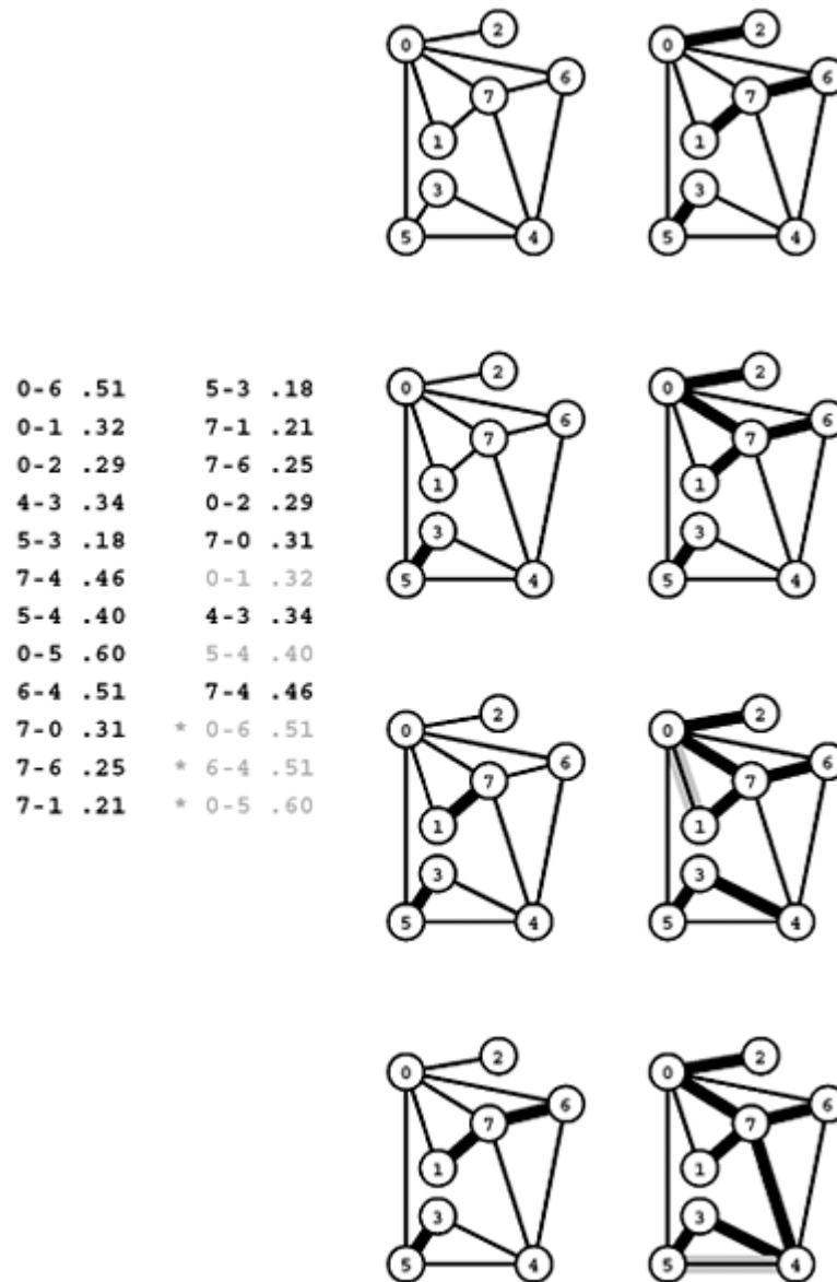
Figure 20.13. Kruskal's MST algorithm
