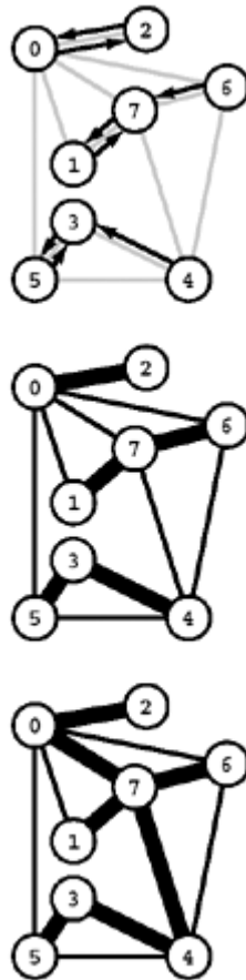
Figure 20.15. Union-find array in Boruvka's algorithm
