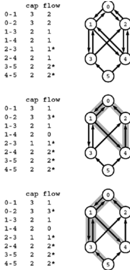
Figure 22.45. Spanning tree for dummy maxflow
