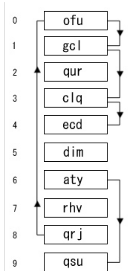
Coalesced Hashing example. For purposes of this example, collision buckets are allocated in increasing order, starting with bucket 0.
