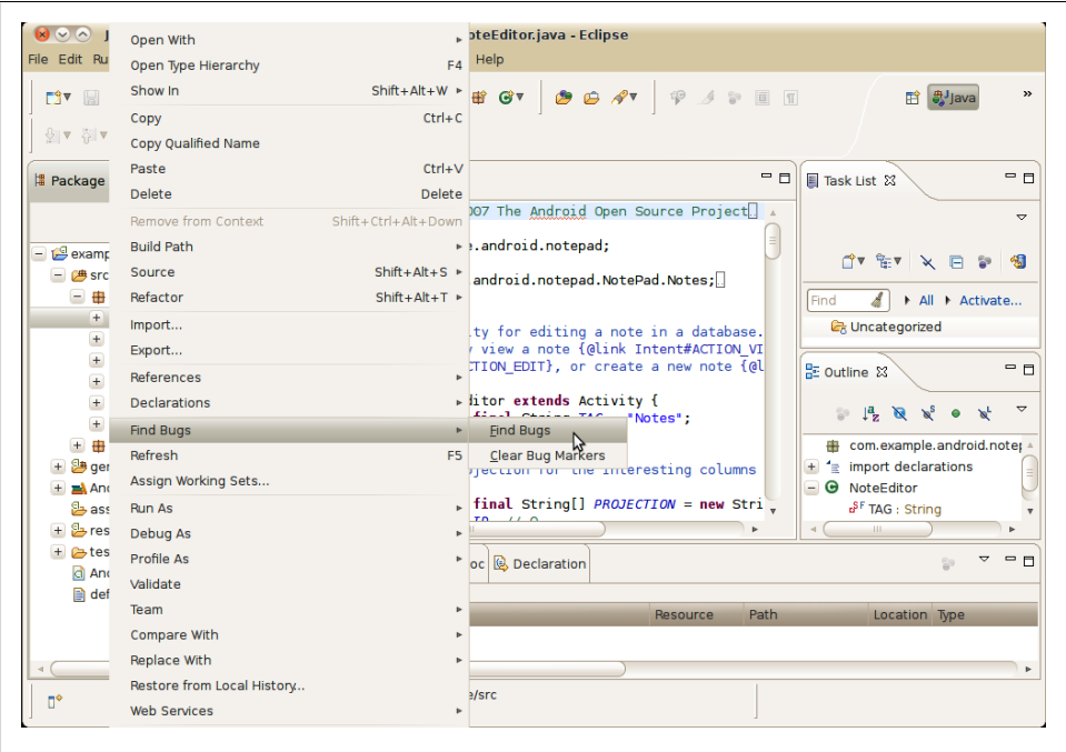
Figure 5-13. Invoking FindBugs
