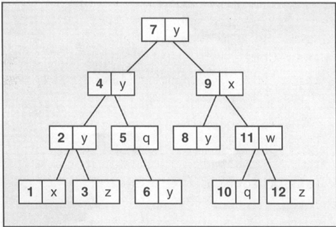
Figure 6.9. Internal Structure of Maps and Multimaps
