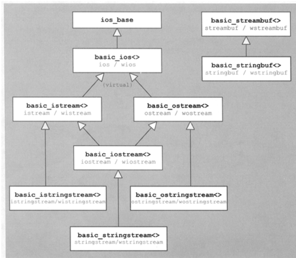
Figure 13.3. Class Hierarchy of the String Stream Classes
