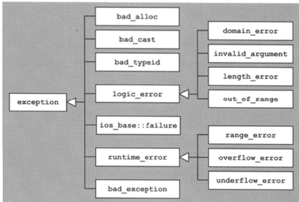
Figure 3.1. Hierarchy of Standard Exceptions
