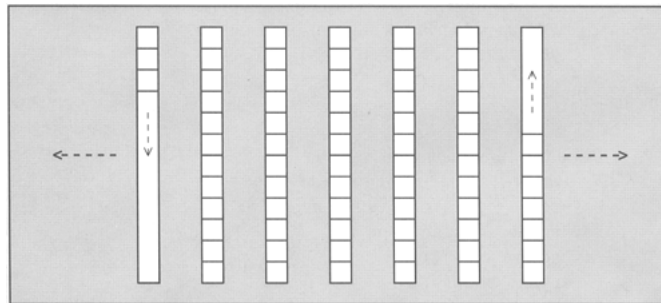
Figure 6.3. Internal Structure of a Deque
