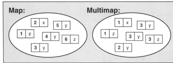
Figure 6.8. Maps and Multimaps
