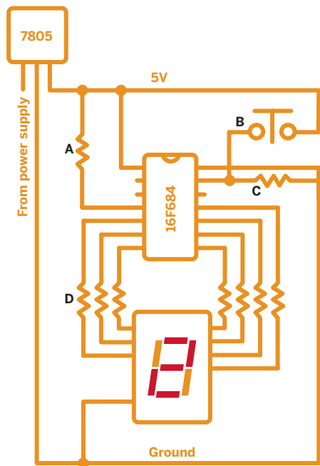
Fig. 1: LED button-press counter circuit: A. 10Ω resistor; B. SPST button; C. 10kΩ resistor; D. 220Ω resistors. Power supply wiring at upper left provides constant voltage from a plug-in transformer.
