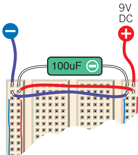
Fig. D: When building circuits around chips, it's convenient to have a positive and negative power supply down each side of your breadboard. For the reaction timer circuit, a 9V supply with a 100 \mu F smoothing capacitor can be set up like this. If your breadboard doesn't color-code the columns of holes on the left and right sides, I suggest you do that yourself with a permanent marker.
